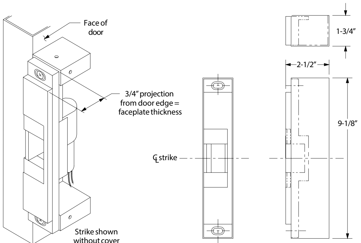
Strike Dimensions and Required Clearances
