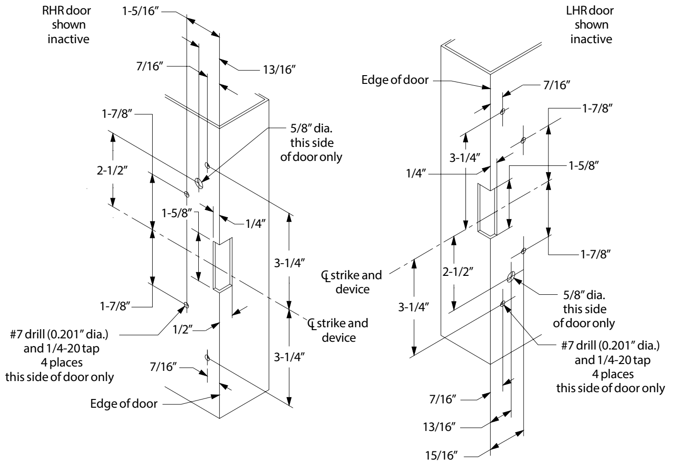
Door Preparation for Strike
